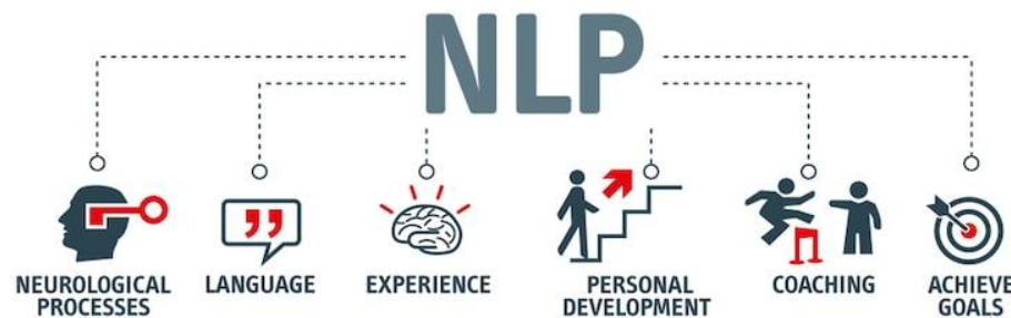
Figure 1. NLP process
